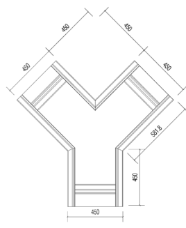
Rear Elevation - open ends - O00
