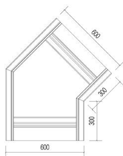
Rear Elevation - open ends - OO
