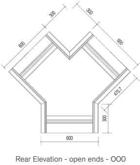
Rear Elevation - open ends - OOO
