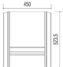
CVI Rear Elevation - open ends - OO
