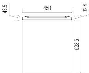
CVI Front Elevation
