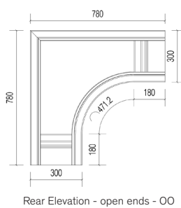
Rear Elevation - open ends - OO
