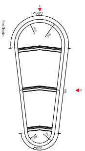
Oval XL AS 2500
