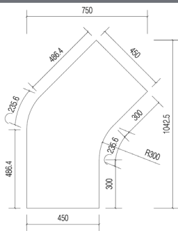
Front Elevation
