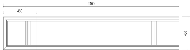
Rear Elevation - one end framed - OF
