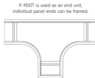
Rear Elevation - one end framed - OOF
