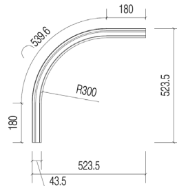
Side Elevation CVI
