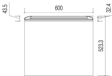
CVI Front Elevation
