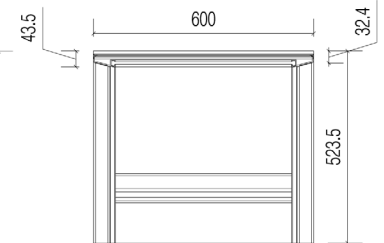
CVE Rear Elevation - open ends - 00
