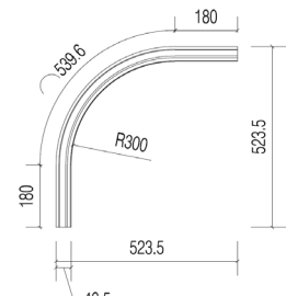
Side Elevation CVE
