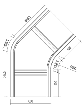
Rear Elevation - open ends - OO
