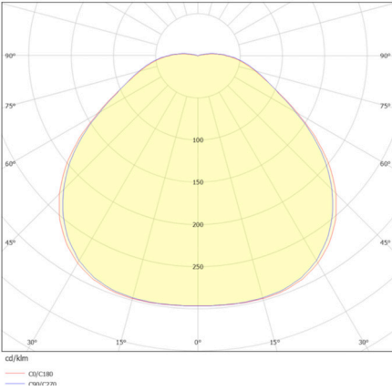
Light distribution curve [cd]
